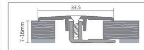
DPS 530 ♦ Suitable for 7-16mm floor ♦ 适用于7-16mm地板
