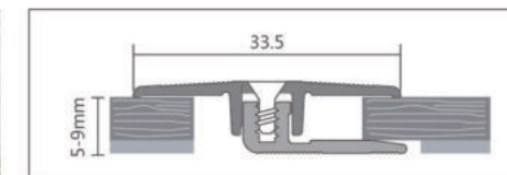
DPS 520 ♦ Suitable for 5-9mm floor ♦ 适用于5-9mm地板
