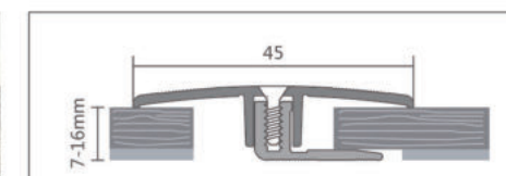
DPS 550 ♦ Suitable for 7-16mm floor ♦ 适用于7-16mm地板
