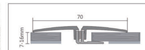
DPS 570 ♦ Suitable for 7-16mm floor ♦ 适用于7-16mm地板
