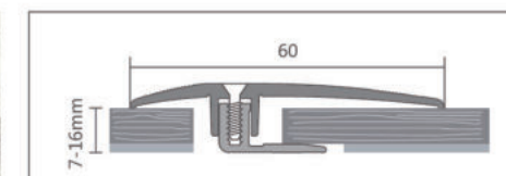
DPS 560 ♦ Suitable for 7-16mm floor ♦ 适用于7-16mm地板
